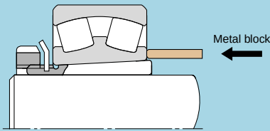
Fig. 15.18 Adapter dismantling
