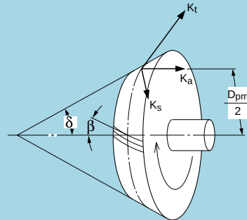
Fig. 6.5 Bevel gear diagram
