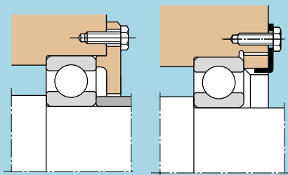
Fig. 14.2 Outer ring clamping
